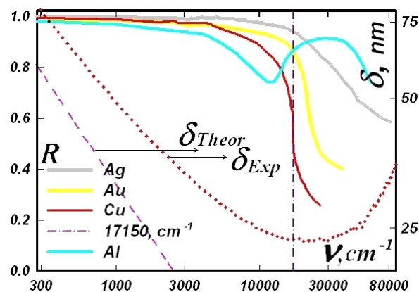
Fig5. Spectral dependences ( 1\ cm^{-1} \approx 3 \cdot 10^{10}\ Hz ) of the reflection coefficients of highly electrically conductive metals (solid lines) and the thickness of the copper skin layer (red dots - experiment, pink dashed line - theory).
