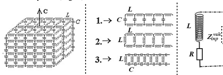
Fig9. Equivalent waveguide circuit of a crystal with layer conductivity: 1 - the electric vector of light incident on the side face is parallel to the C axis, 2 - the electric vector of light incident on the side face is parallel to the conducting layers, 3 - electric vector of light incident on the face perpendicular to the C axis for any of its polarization is parallel to the conducting layers.
