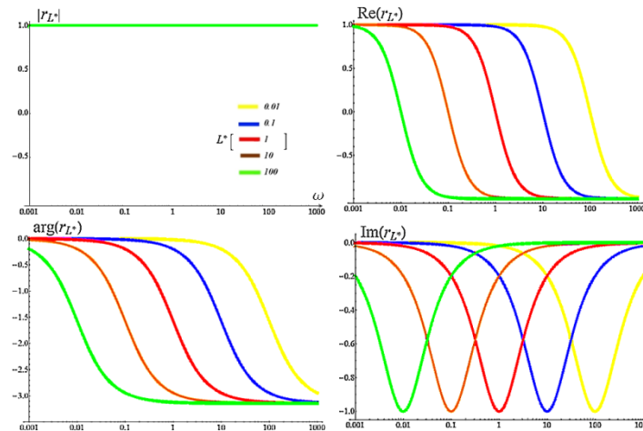
Fig10. Spectra of the components of the complex reflection coefficient of the reduced inductances of various sizes
