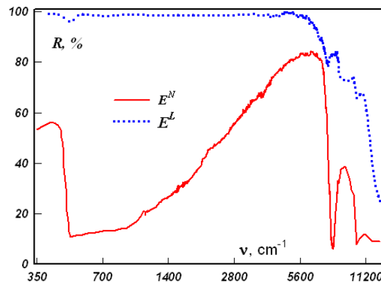
Fig3. Spectra of normal reflection modelling nanostructures at orientation of electric vector E in parallel ( E^L ) and it is perpendicular ( E^N ) to metal strings.
