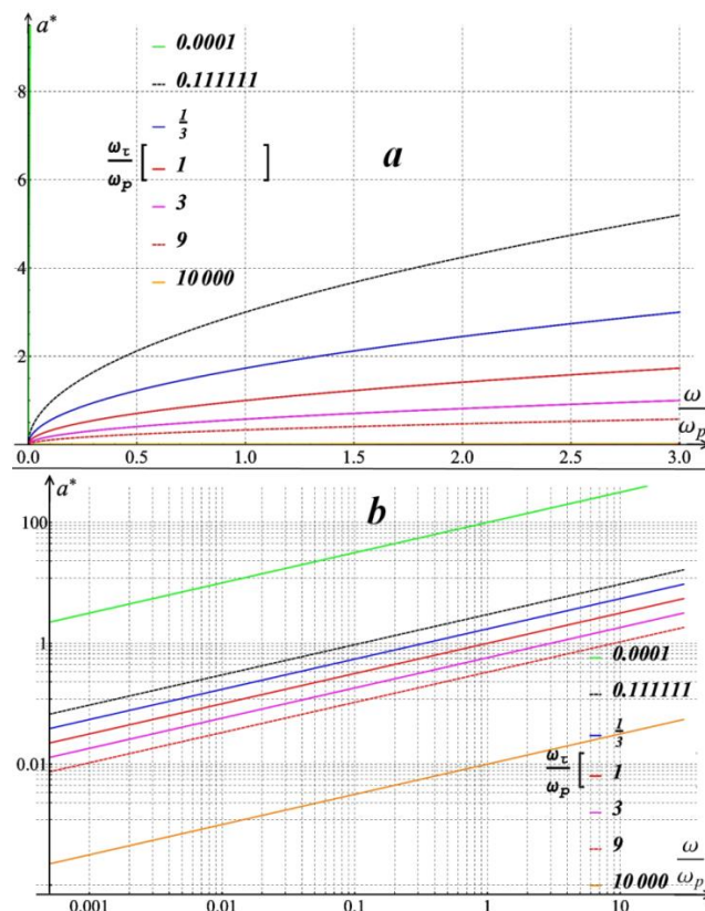
Fig7. Frequency dependence of the "absorption" of the skin layer (skin absorption)
