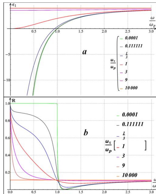
Fig1. Dependence of the real part of the dielectric constant \epsilon_1 (a) and the reflection coefficient R on the reduced frequency \omega/\omega_p at different values of the relative attenuation \omega_\tau/\omega_p of the free carrier plasma
