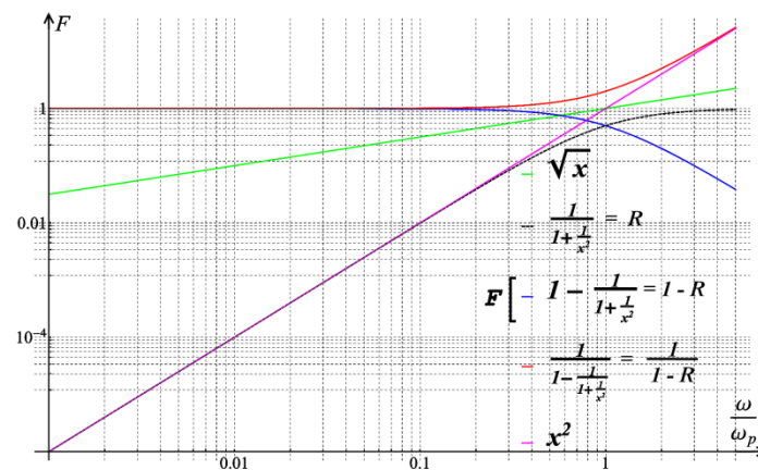
Fig8. Frequency dependence of skin reflection and its corrections / factors
