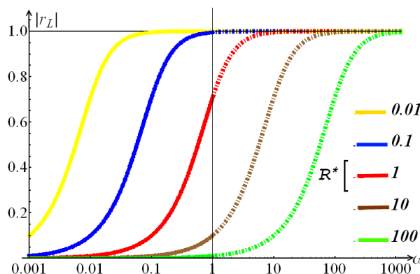
Fig11. Reflectance spectra of a unit reduced inductance at different resistivities (reduced to vacuum impedance).
