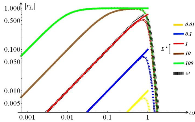
Fig13. Clipping of the reflection spectra of various inductances at a unit reduced resistivity at the plasma frequency
