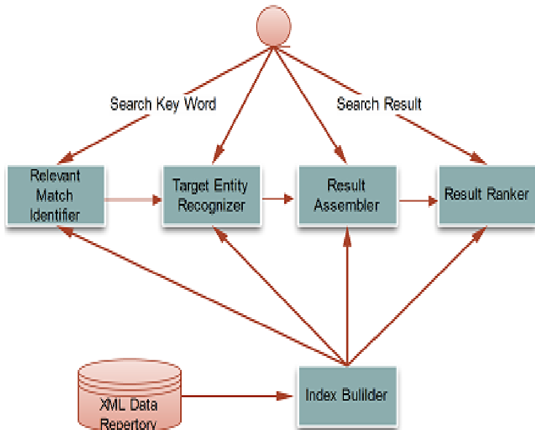
Fig3: Architecture of XSearch
