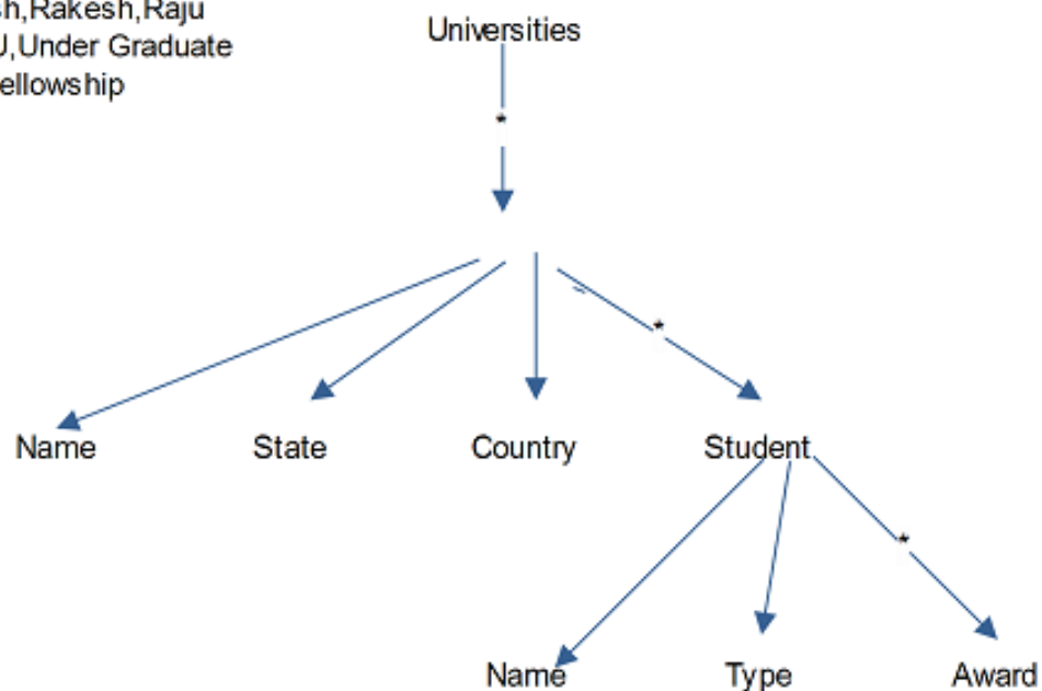
Fig 1.Schema of an XML Document
