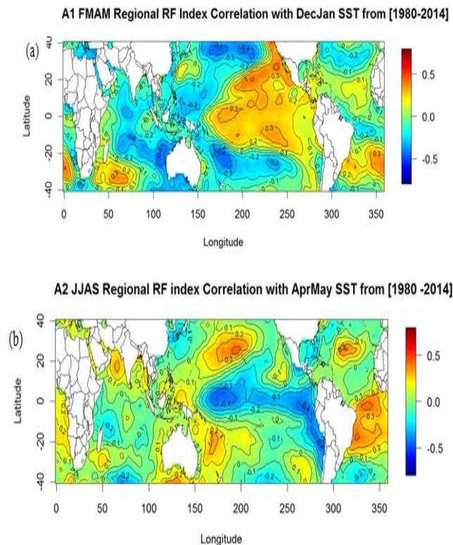
Figure3. Regional R_k index correlation with global spatial SSTa
