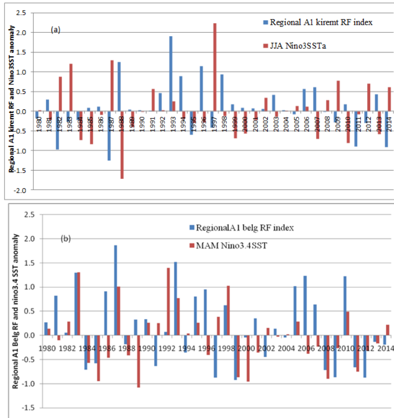
Figure 4. Regional rainfall and Niño regions SST anomaly during rainy seasons
