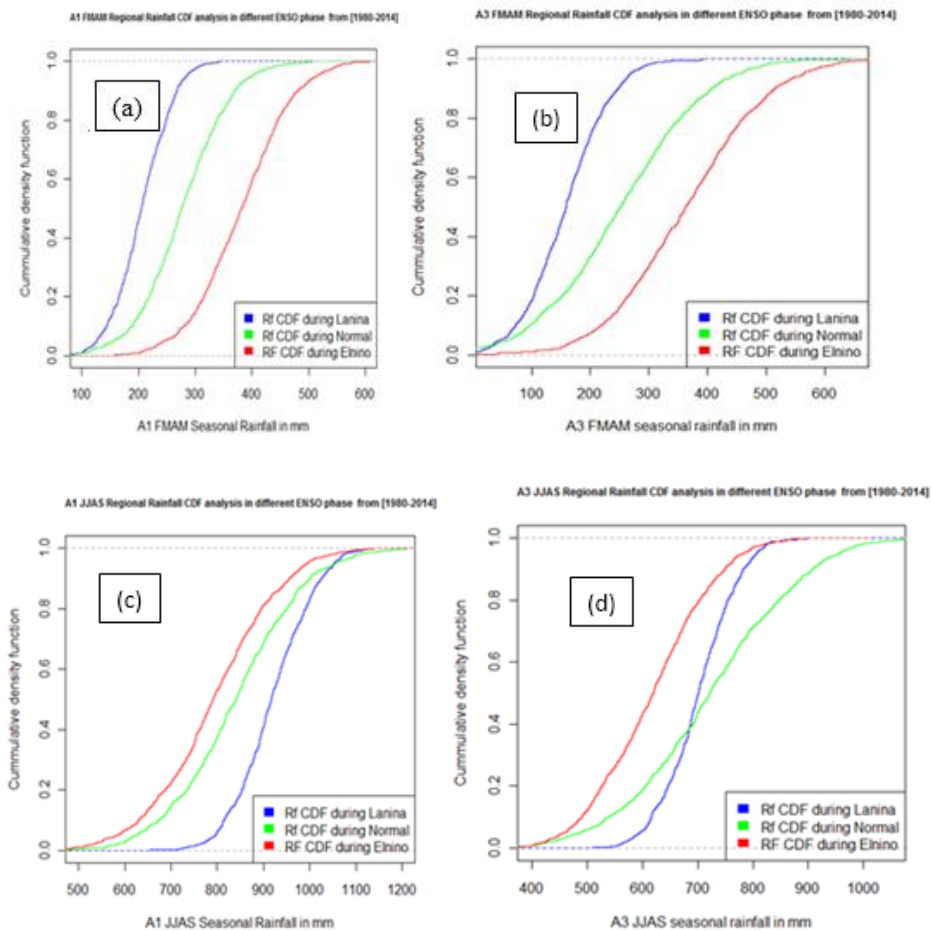
Figure 5. comparison of cumulative seasonal rainfall at various ENSO phases
