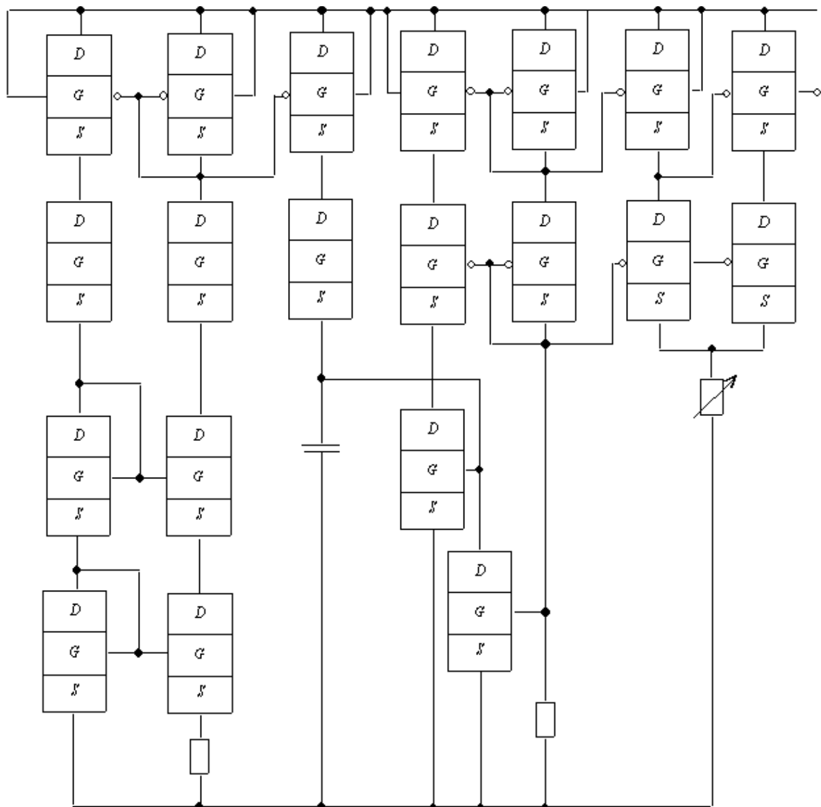
Fig1a. Structure of the considered voltage reference [19]
