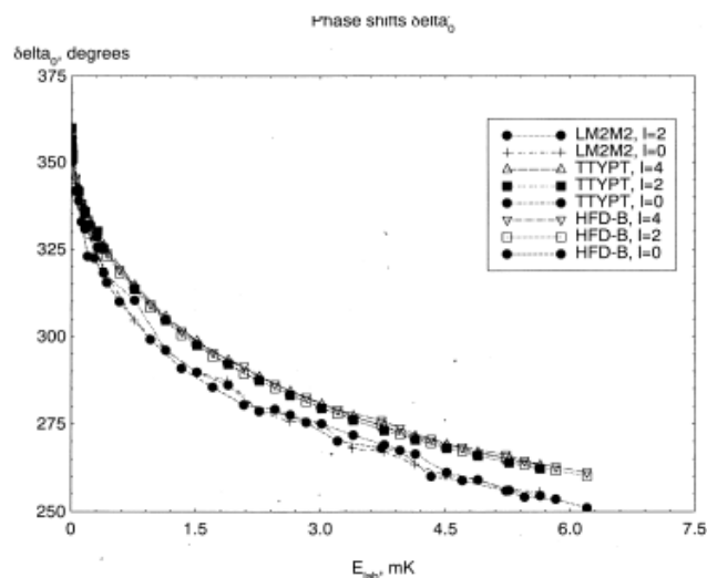
Figure4. Dependence of phase shifts on energy for the collisions between helium atom and molecule for potentials HFD – B, LM2M2, TTY P[32] calculated (a) without and (b) with taking into account the hard core
