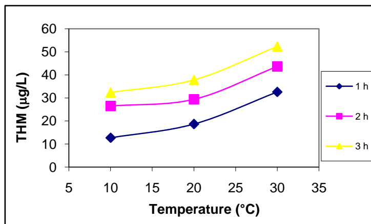
Fig2. The effect of temperature in the formation of THMs
