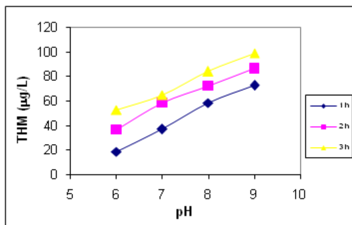
Fig3. The impact of pH in the formation of THMs
