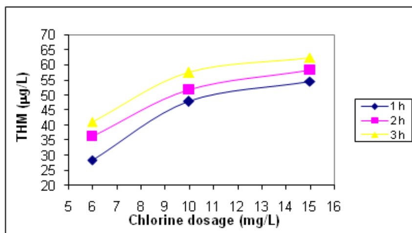
Fig4. The impact of chlorine dosage in the formation of THMs
