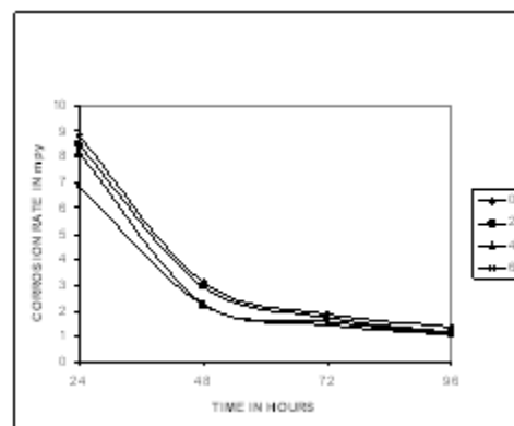
Fig3. Weight loss corrosion in 3.5% sodium chloride solution
