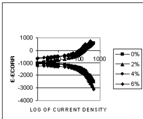
Fig8. Potentiostat test in 0.35 % sodium chlorides solution
