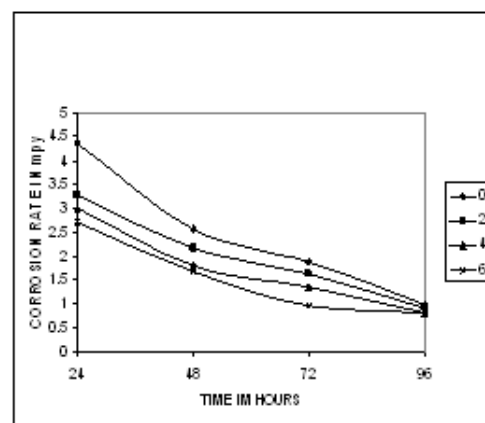
Fig2. Weight loss corrosion in 0.35% sodium chloride solution
