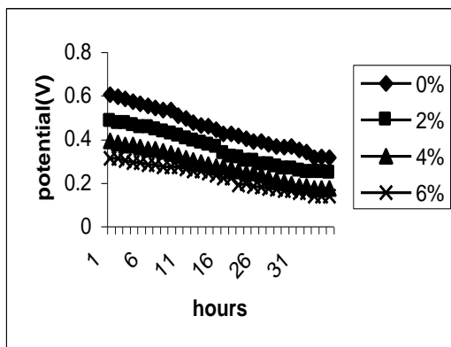
Fig5. Open circuit potential test in 0.35 % sodium chlorides solution
