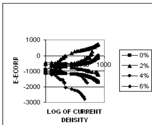
Fig9. Potentiostat test in 3.5 % sodium chlorides solution
