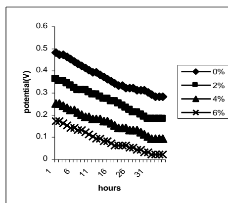
Fig4. Open circuit potential test in 0.035% sodium chloride solution
