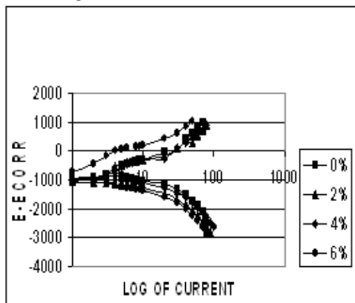
Fig7. Potentiostat test in 0.035 % sodium chlorides solution
