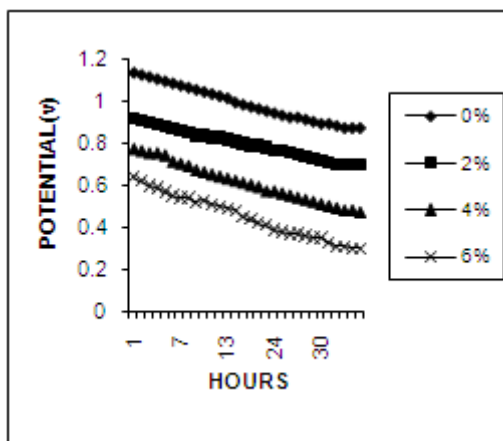
Fig6. Open circuit potential test in 3.5 % sodium chlorides solution
