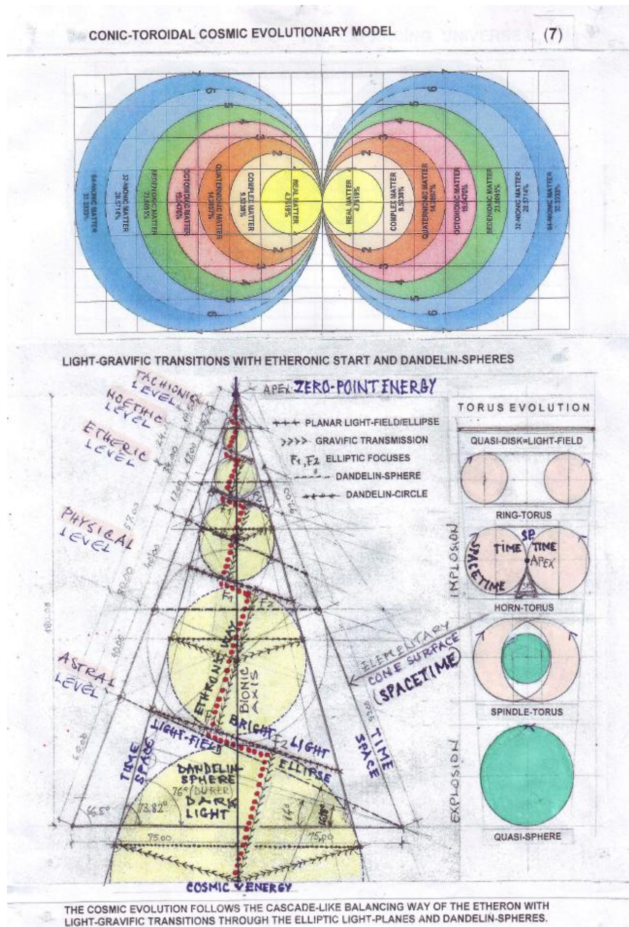
Fig (7) – Conic-toroidal Cosmic Evolutionary Model
