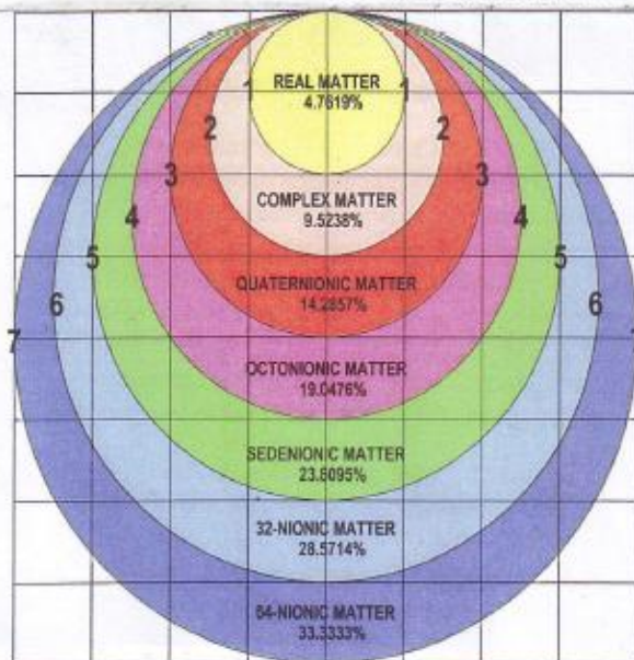
Fig (11) – Overview of the Bionic and Nucleonic Structured Sections
