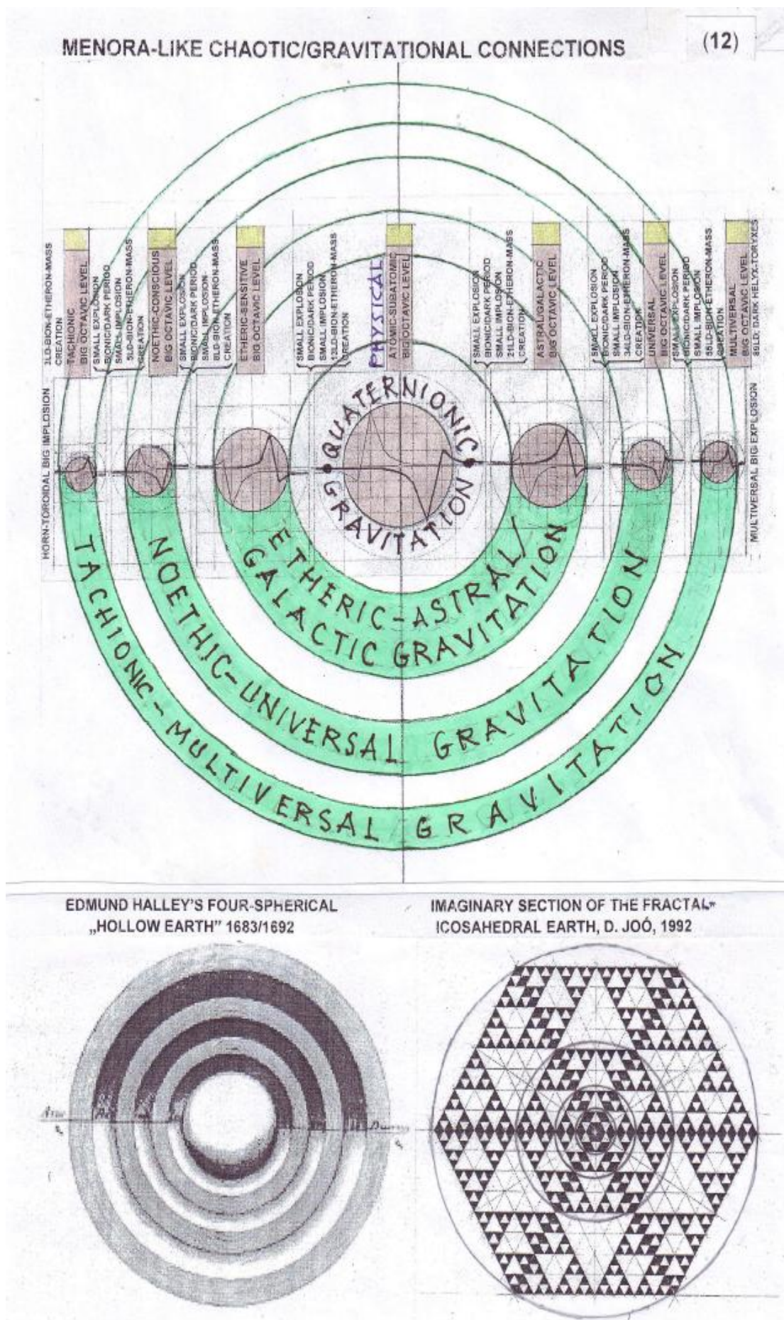
Fig (12) – Menora-like Chaotic-gravitational Connections.
