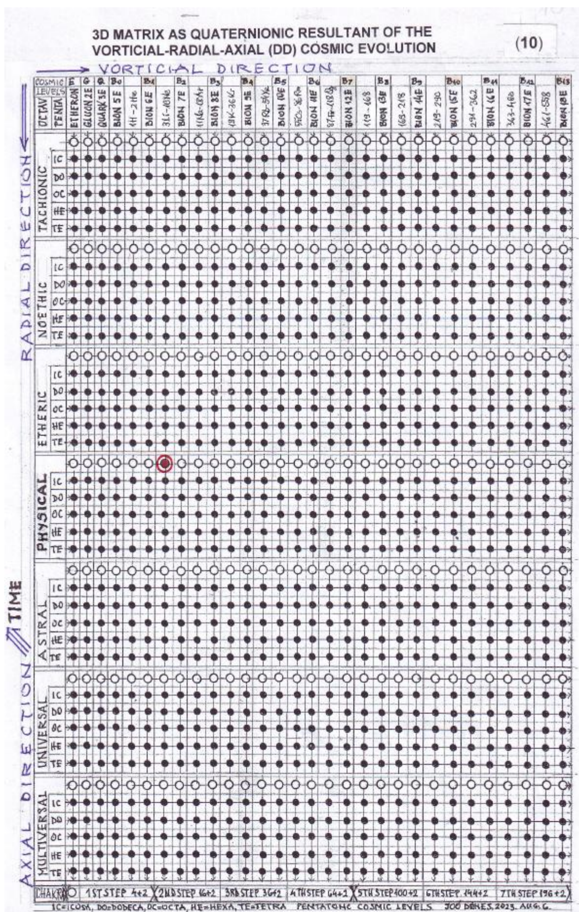
Fig (10) – 3D Matrix as Quaternionic Resultant of the Vorticial-radial-axial (DD) Cosmic Evolution
