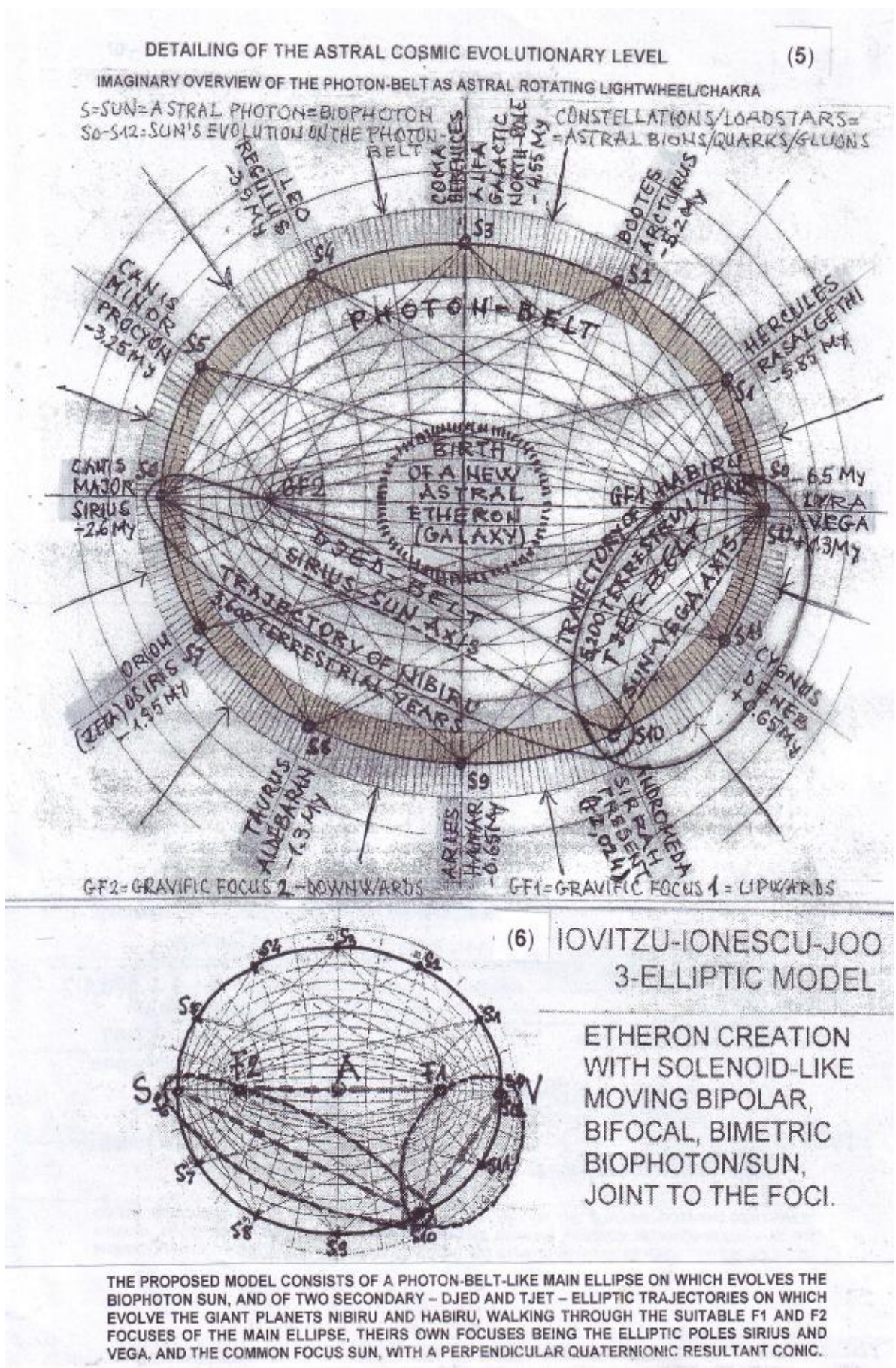
Fig (5) – Detailing of the Astral Cosmic Evolutionary Level
