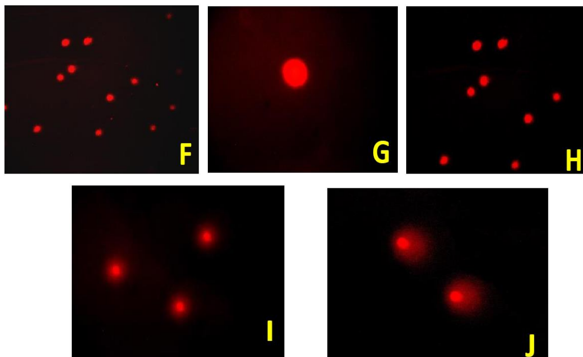
Figure 6. Determination of the toxic effects of increasing doses of NiO NPs on the DNA structure of human blood leukocytes by comet assay. (F-G) Control group; (H) 10 µg/mL NiO NP applied group; (I) 100 µg/mL NiO NP applied group; (J) 1000 µg/mL NiO NP applied group.
